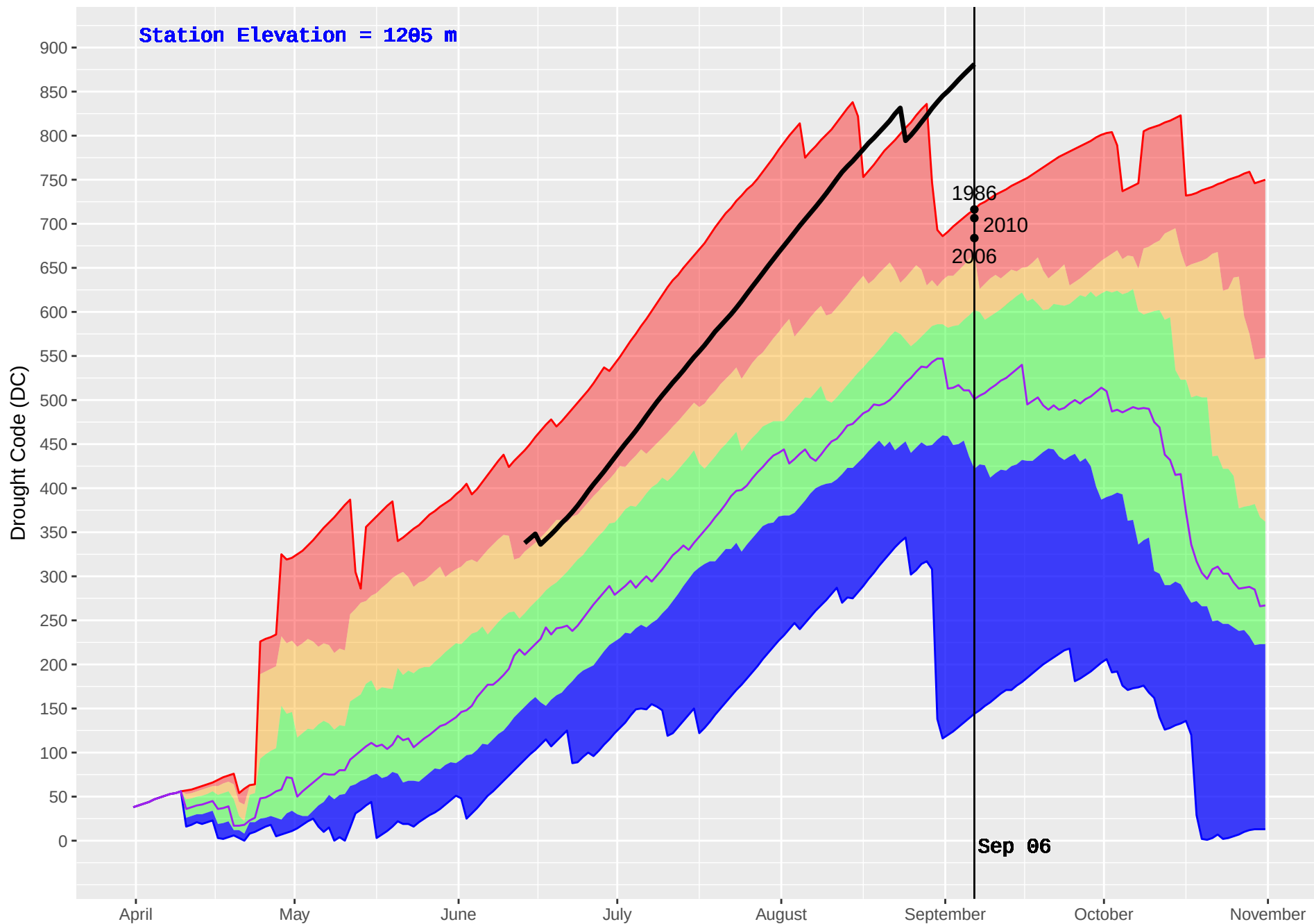
GWYNETH LAKE (309) : Historical (1986–2016) and Current (2017) Noon Drought Code (DC)
